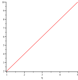
Figure 1. A plot of the price V(\eta) with boundary conditions V(1) = 2 and V(5) = 10 .
